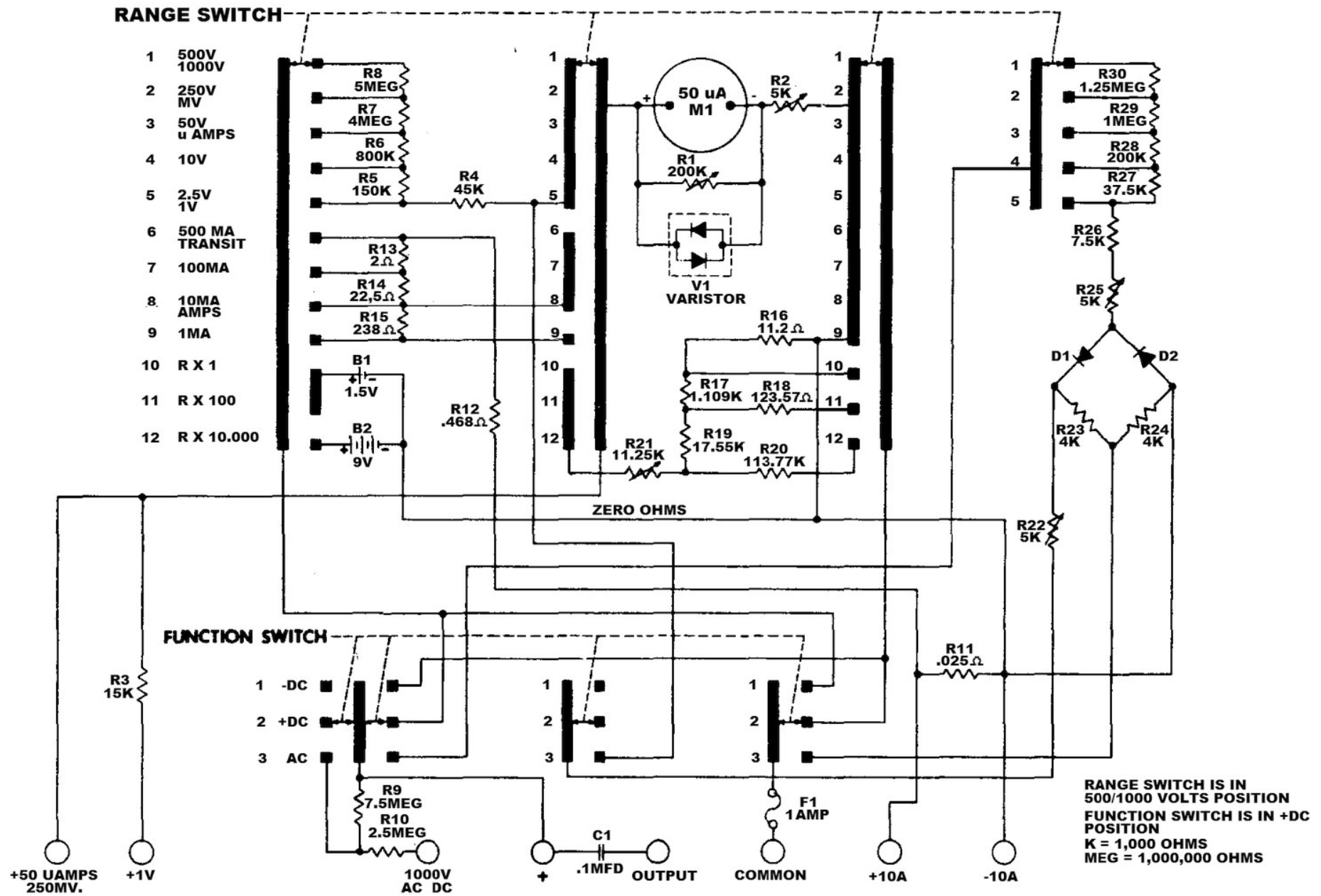
SCHEMATIC DIAGRAM
